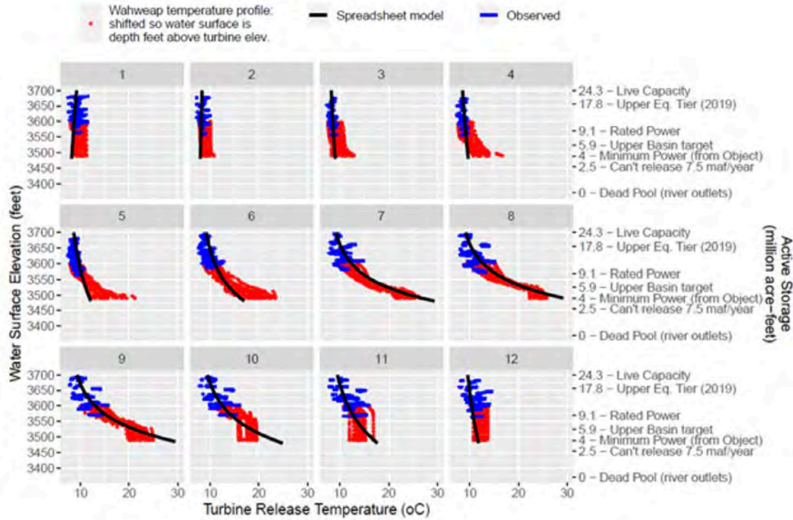
Figure A2. Compare observed penstock release temperature (blue) and translated depth-temperature profile data (red). Black lines show estimated release by an empirical spreadsheet model (Dibble et al., 2020).
