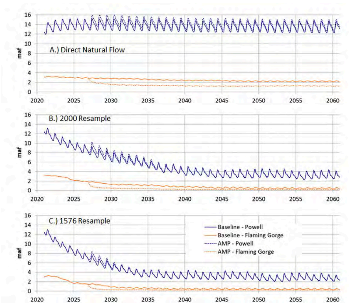
Figure 9.27. Average storage volumes of Flaming Gorge Reservoir and Lake Powell with the Flaming Gorge to Powell Backup alternative. (A) using the optimistically wet DNF hydrologic scenario. (B) using the Millennium Drought scenario (2000 Resample), and (C) using the Paleo Tree Ring Drought (1576 Resample) hydrologic conditions.
