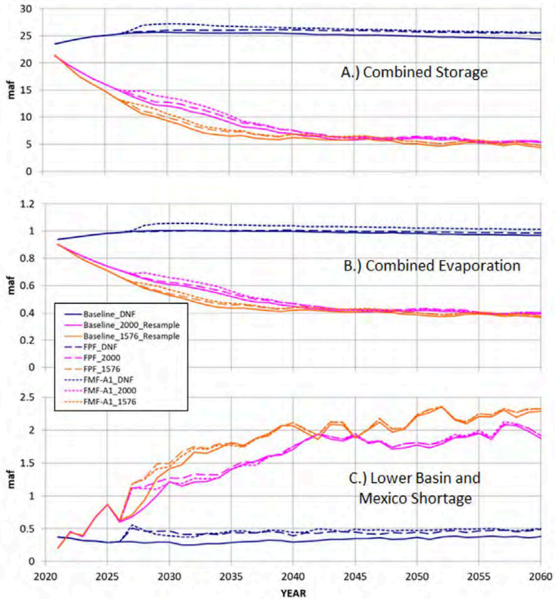
Figure 9.15. Comparison of FMF-1A and FPF Management Alternatives when using average values from hydrologic traces of the Millennium Drought (2000 Resample), Paleo Tree Ring Drought (1576 Resample), and DNF hydrology. (A) shows combined storage of Lake Mead and Lake Powell; (B) shows combined evaporation from Lake Mead and Lake Powell. (C) shows total Lower Basin and Mexico shortages.
