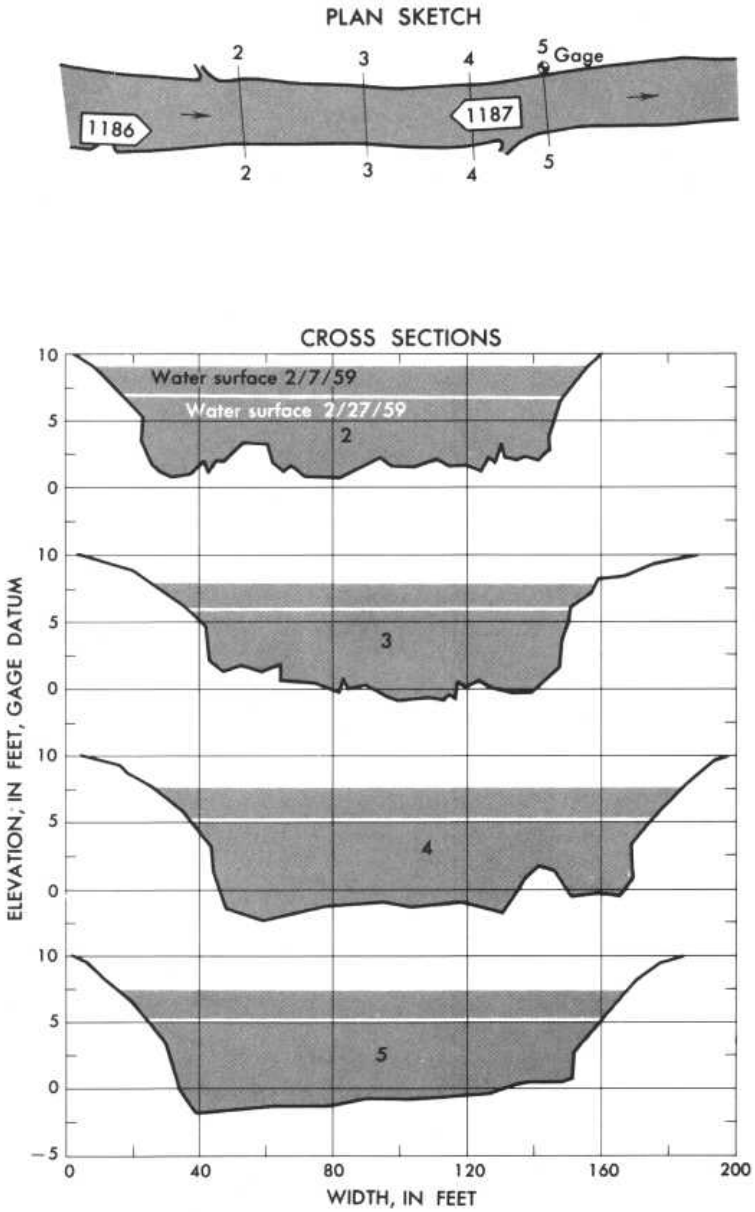
Plan sketch and cross sections, Chattahoochee River near Leaf, Ga.
