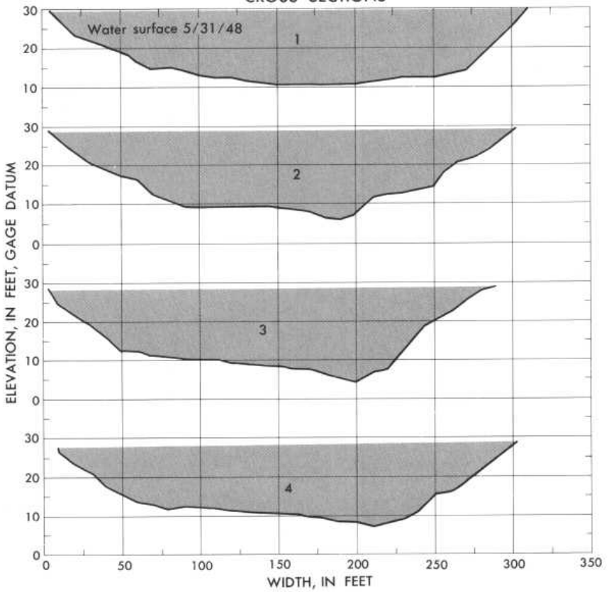
Plan sketch and cross sections, Spokane River at Spokane, Wash.
