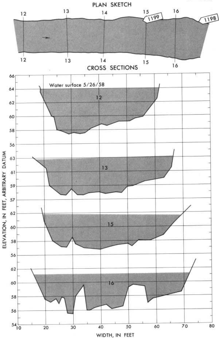
Plan sketch and cross sections, Clear Creek near Golden, Colo.
